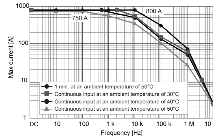
Figure 1. Frequency Derating
